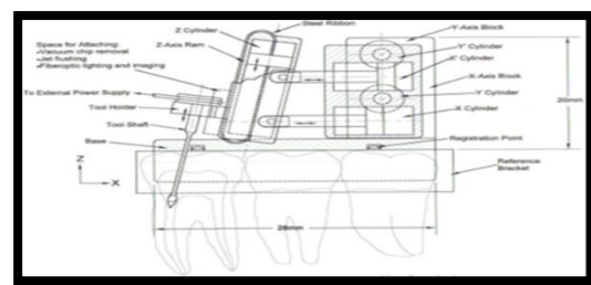
Figure 2: Micro-robot conceptual design. [6]
