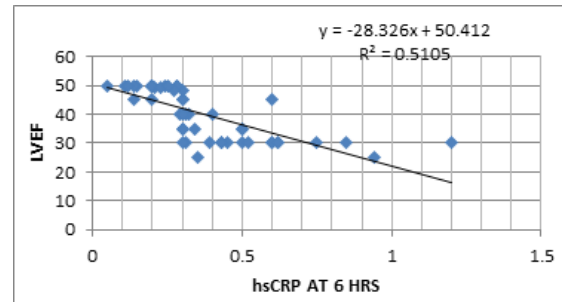
Figure 1: Pearson Correlation between Lvef and hsCRP
