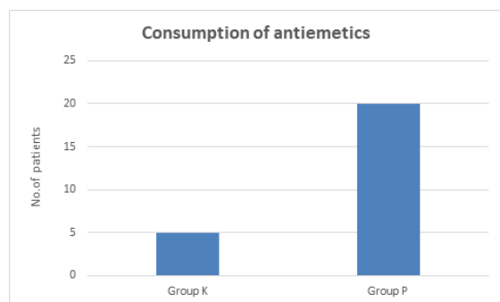
Figure 1: Consumption of antiemetics in study groups.
